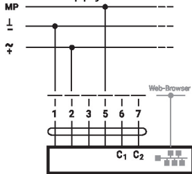
M-Bus with converter
