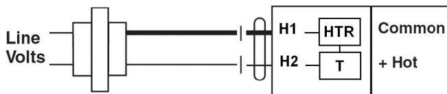
NEMA 4 Heater Option 24 VAC Transformer
