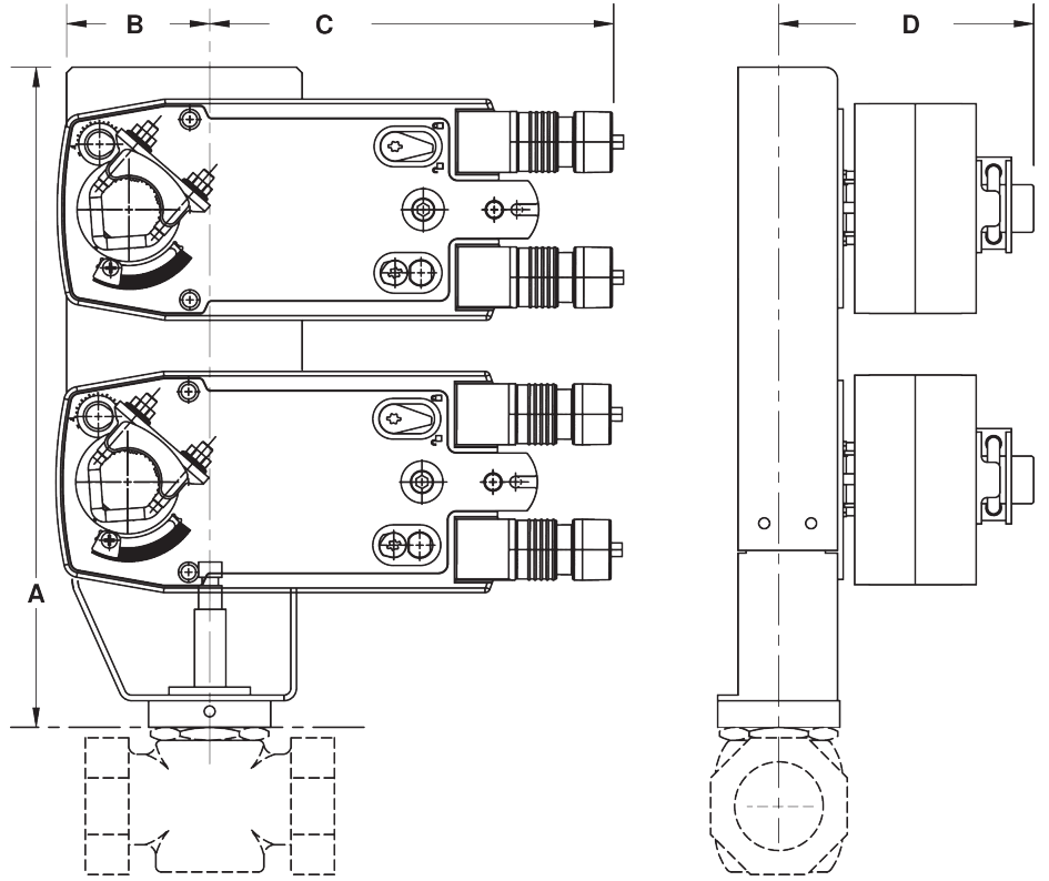
Dimensional drawings
