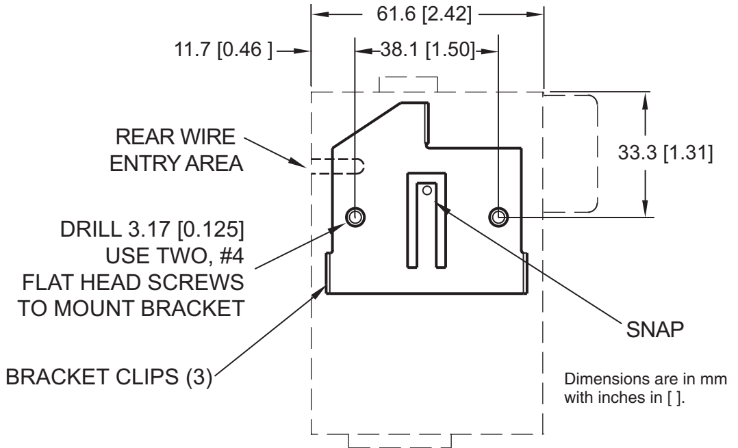
Figure 2.2 Wall Mounting
