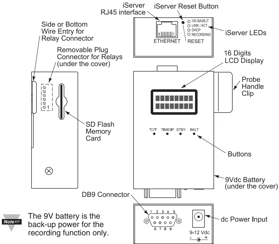
Figure 2.3 Parts of the iServer Unit
