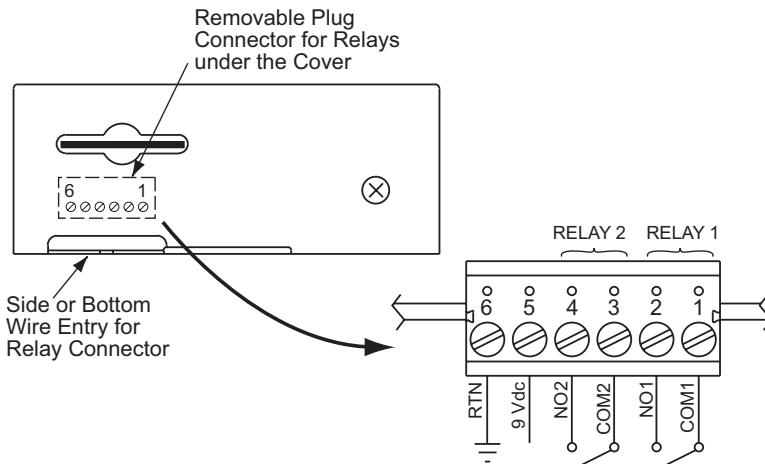
Figure 2.6 Relay Connections
