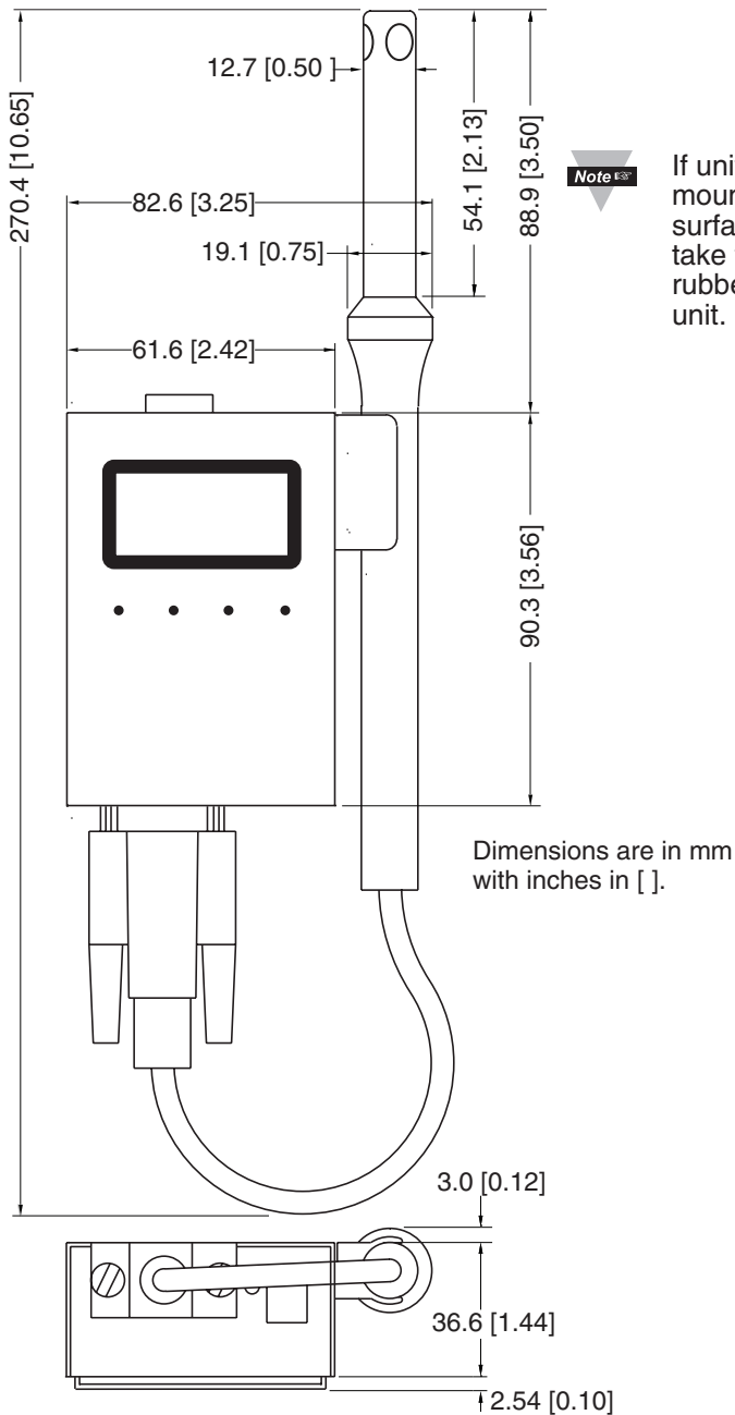
Figure 2.1 Dimensions
