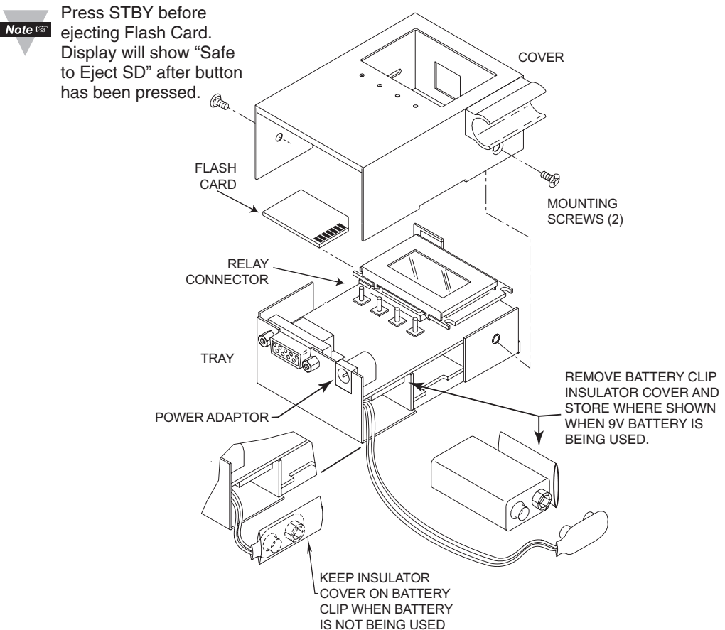
Figure 2.4 Opening the Unit
